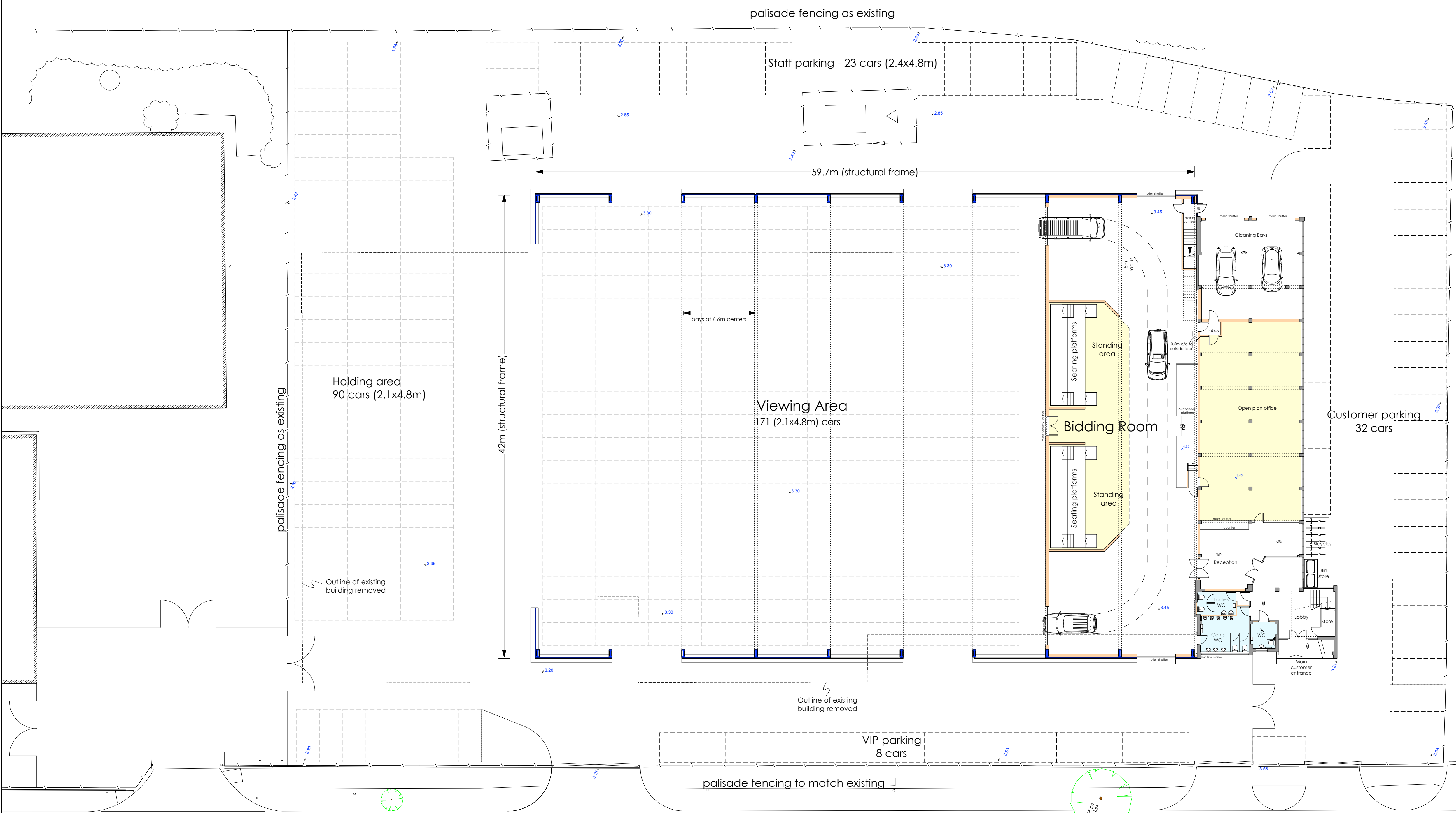
Ground Floor and site layout
