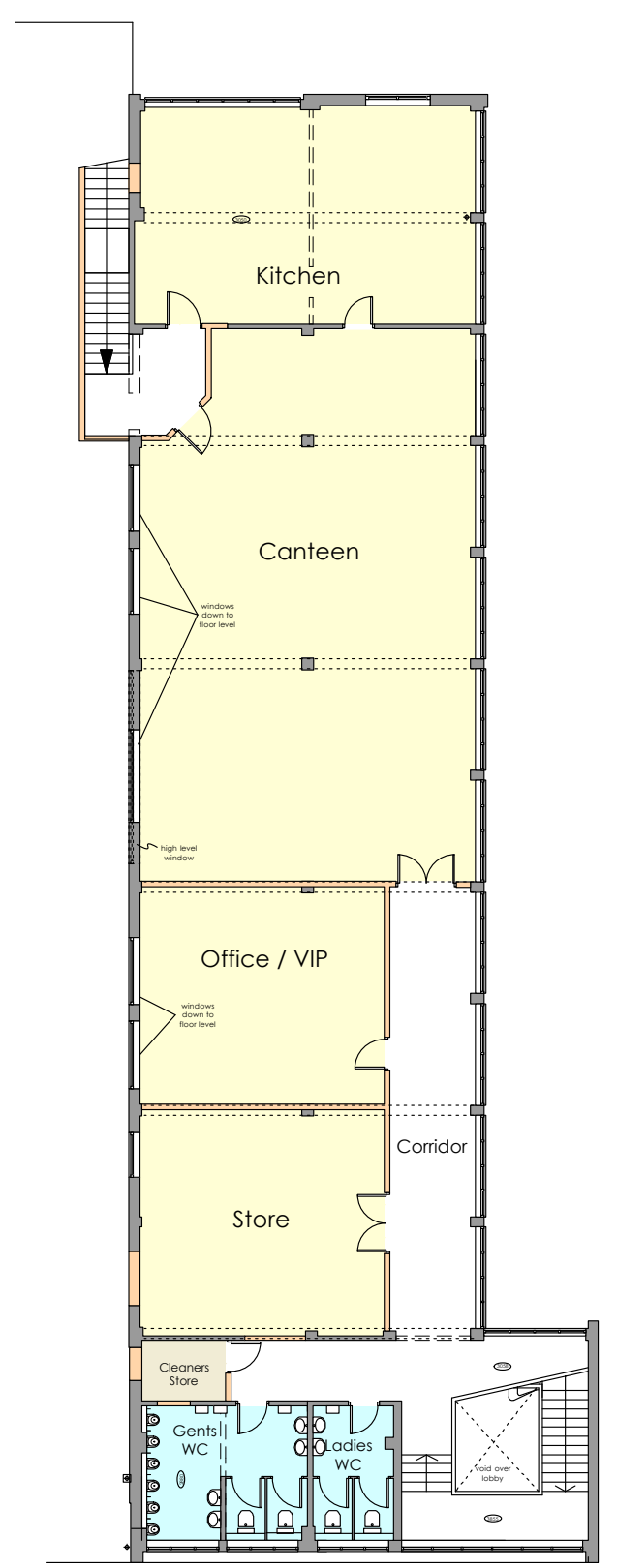
First Floor
